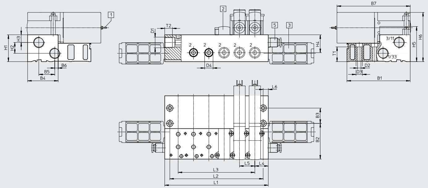
[1] Plug vanes or moulded-in cable [2] Cover plate [3] Silencer [5] Push-in fitting
