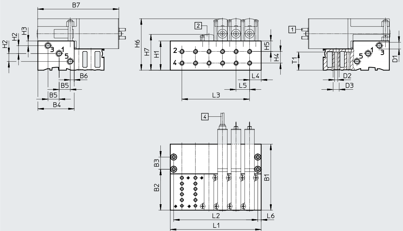
[1] Plug vanes
